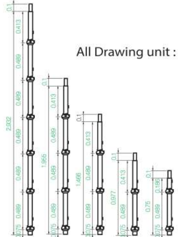
CUPLOCK SYSTEM (STANDARD)
